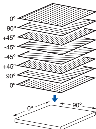
■ Quasi-isotropic lay-up
