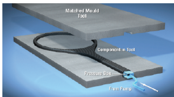
Pressure bag process
