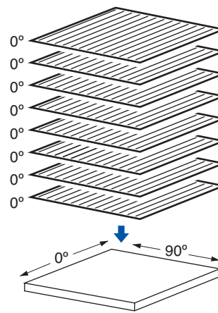
■ Unidirectional lay-up
