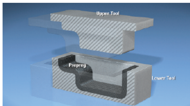
Match moulding process
