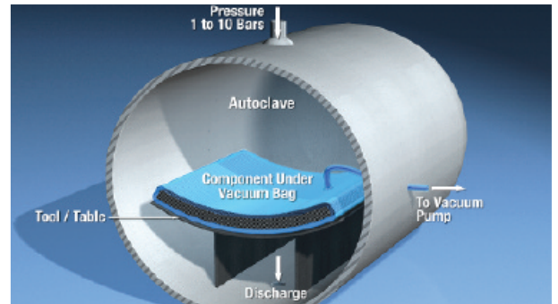
Autoclave process
